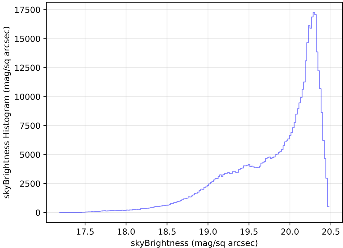
weather_cloudso2v3.4_10yrs WFD i band: skyBrightness Histogram
