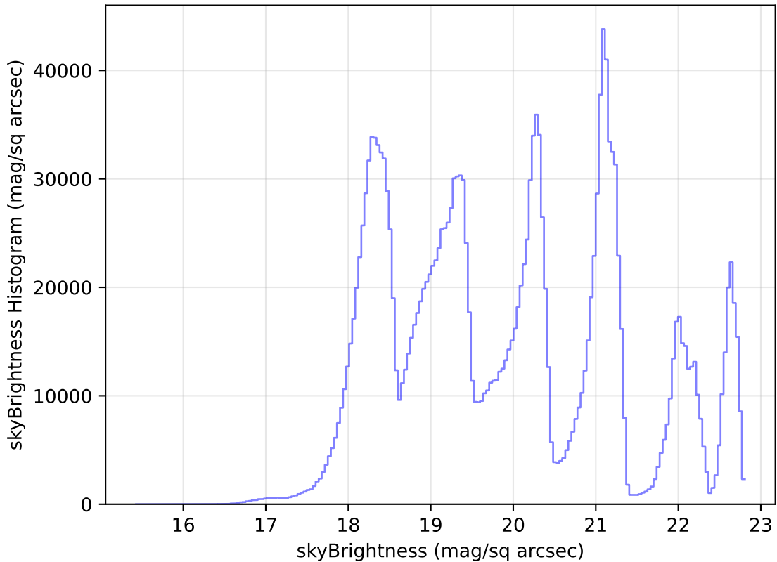
weather_cloudso2v3.4_10yrs WFD all bands: skyBrightness Histogram
