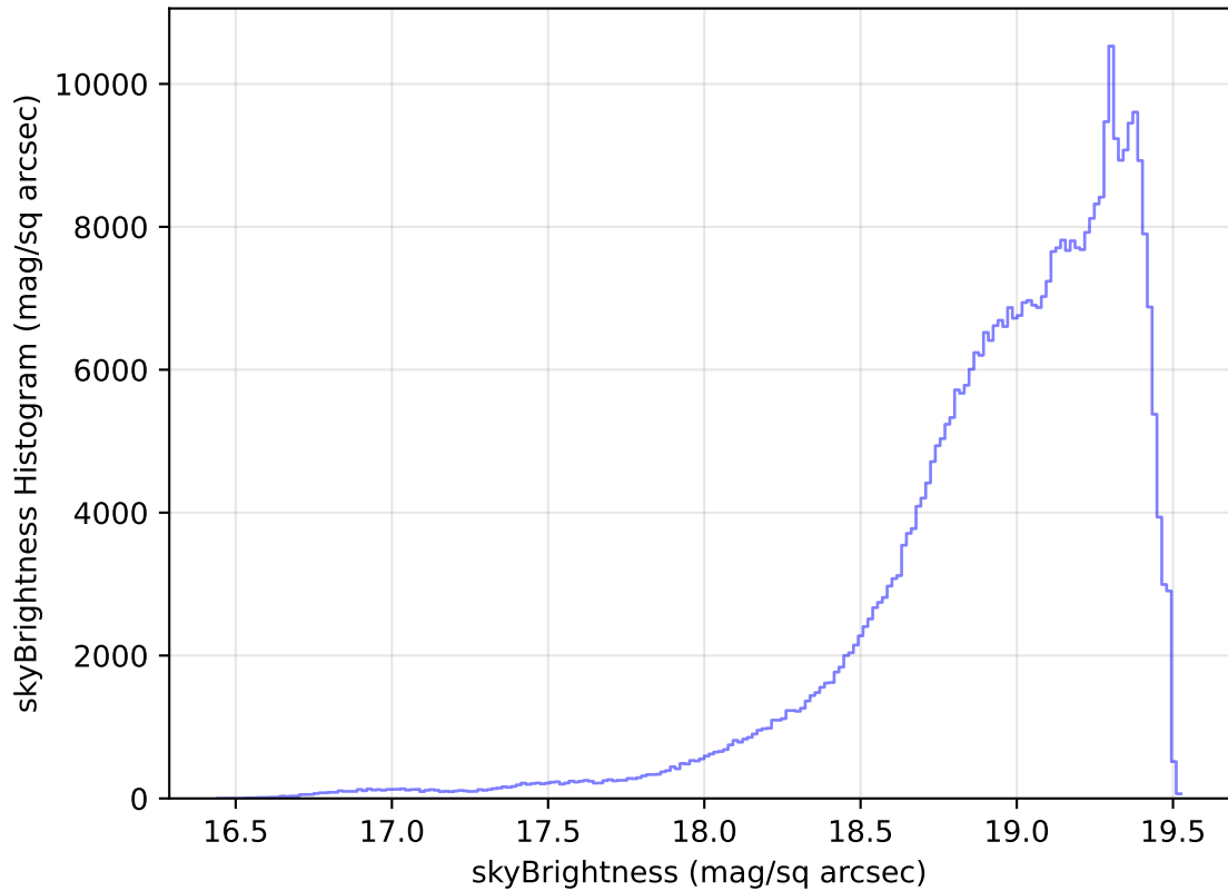
weather_cloudso2v3.4_10yrs All sky z band: skyBrightness Histogram
