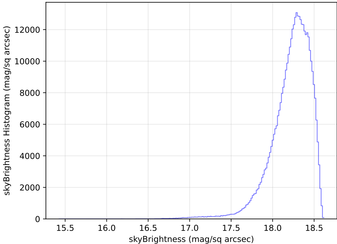
weather_cloudso2v3.4_10yrs All sky y band: skyBrightness Histogram
