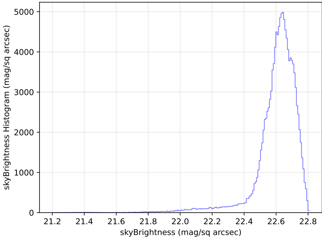
weather_cloudso2v3.4_10yrs All sky u band: skyBrightness Histogram
