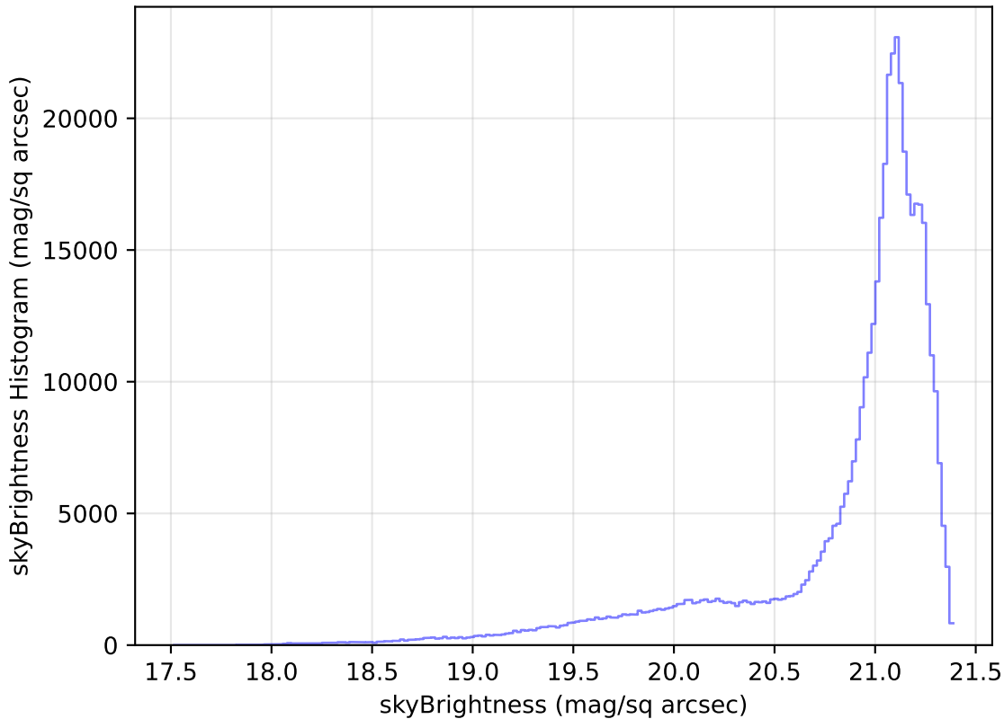
weather_cloudso2v3.4_10yrs All sky r band: skyBrightness Histogram
