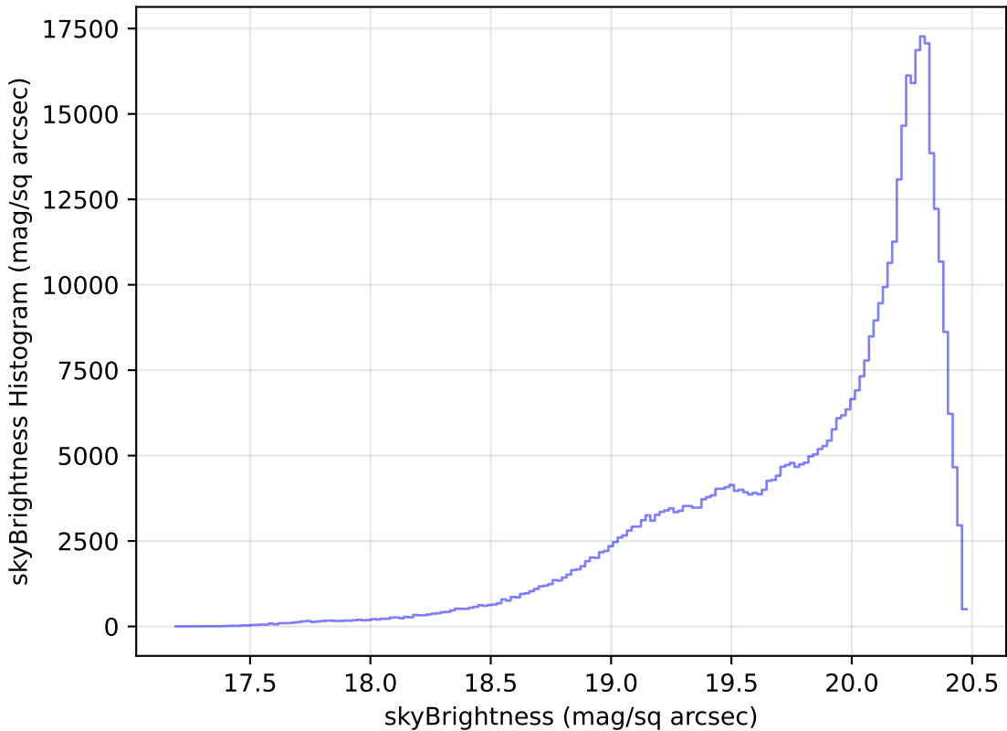
weather_cloudso2v3.4_10yrs All sky i band: skyBrightness Histogram
