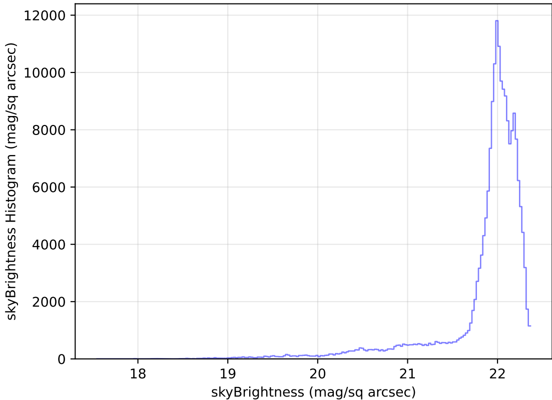
weather_cloudso2v3.4_10yrs All sky g band: skyBrightness Histogram
