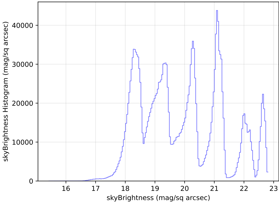
weather_cloudso2v3.4_10yrs All sky all bands: skyBrightness Histogram
