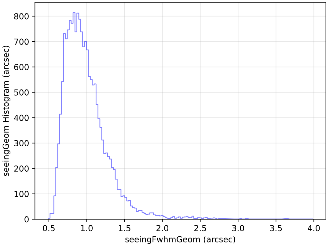
weather_cloudso2v3.4_10yrs Yr 1 u band: seeingGeom Histogram
