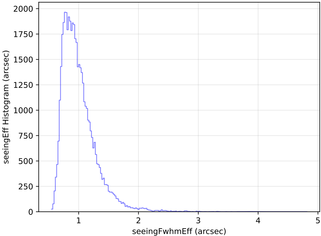
weather_cloudso2v3.4_10yrs Yr 1 z band: seeingEff Histogram
