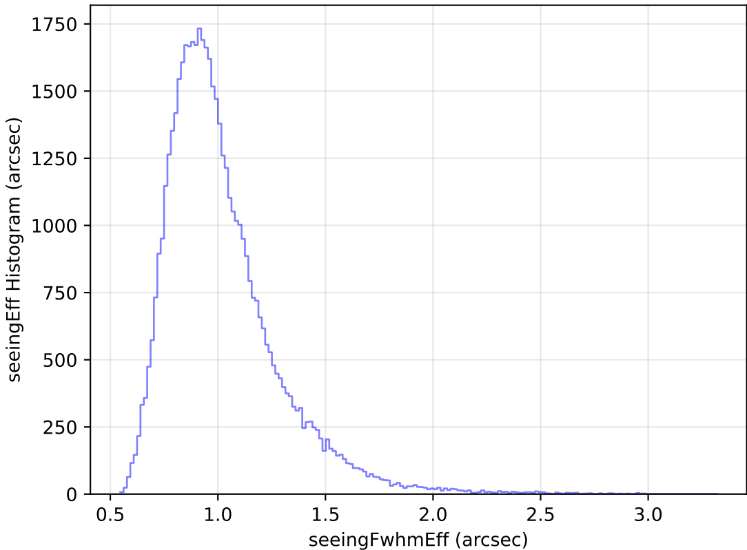
weather_cloudso2v3.4_10yrs Yr 1 y band: seeingEff Histogram
