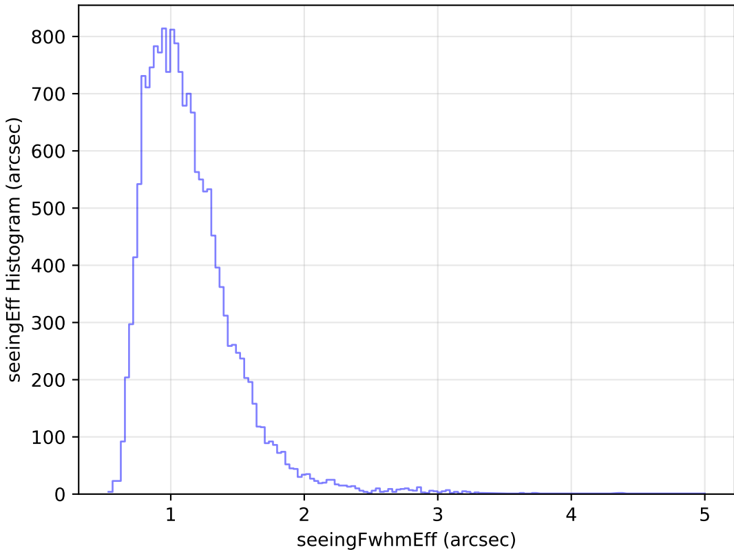
weather_cloudso2v3.4_10yrs Yr 1 u band: seeingEff Histogram
