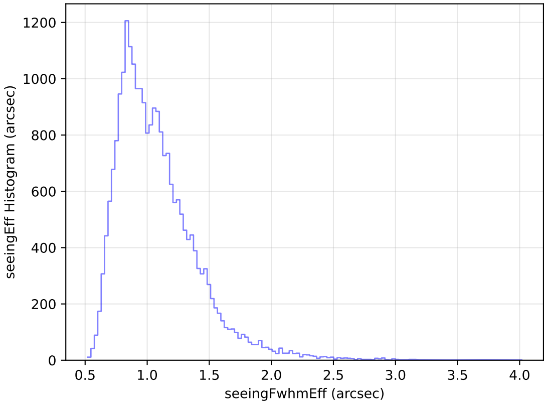
weather_cloudso2v3.4_10yrs Yr 1 g band: seeingEff Histogram
