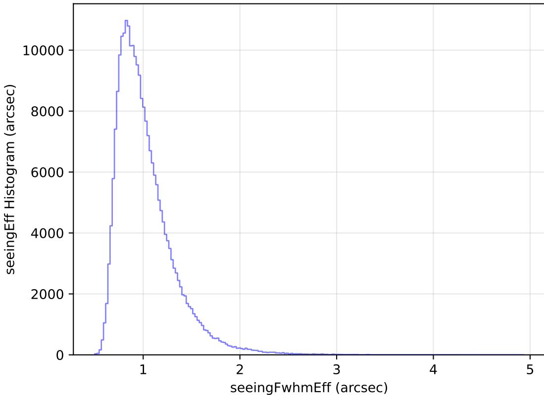
weather_cloudso2v3.4_10yrs Yr 1 all bands: seeingEff Histogram
