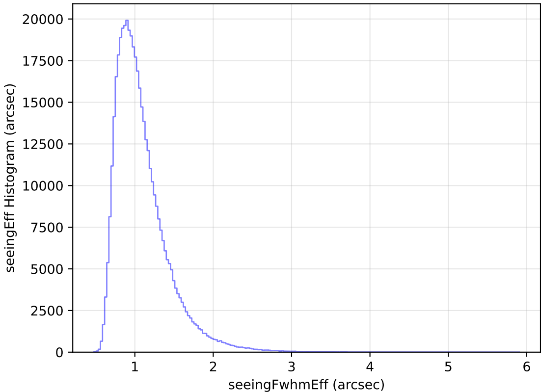
weather_cloudso2v3.4_10yrs WFD z band: seeingEff Histogram
