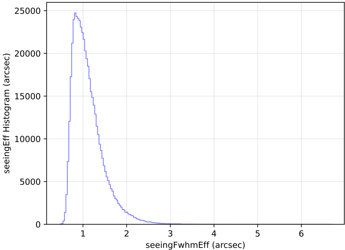
weather_cloudso2v3.4_10yrs WFD r band: seeingEff Histogram
