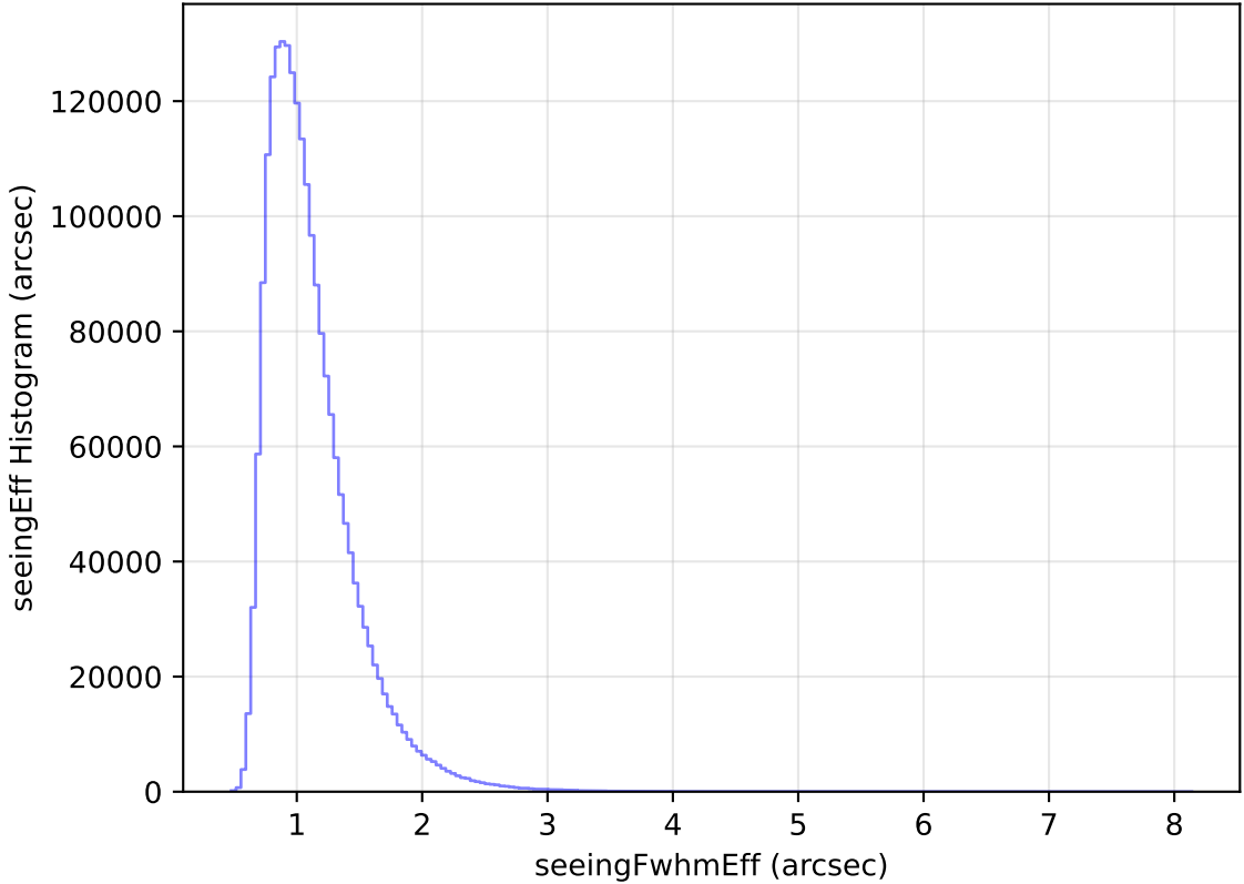
weather_cloudso2v3.4_10yrs WFD all bands: seeingEff Histogram
