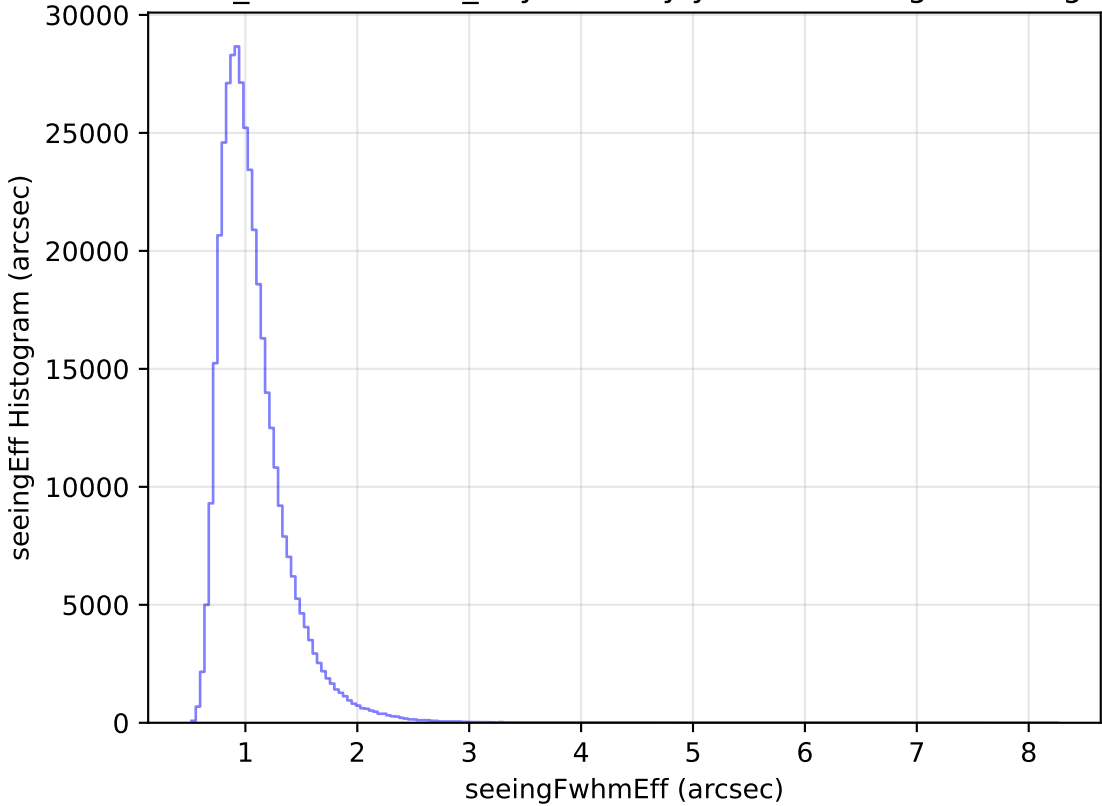
weather_cloudso2v3.4_10yrs All sky y band: seeingEff Histogram
