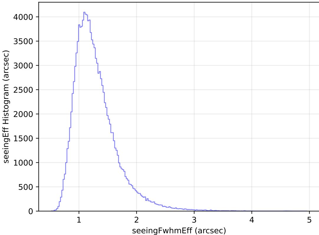
weather_cloudso2v3.4_10yrs All sky u band: seeingEff Histogram
