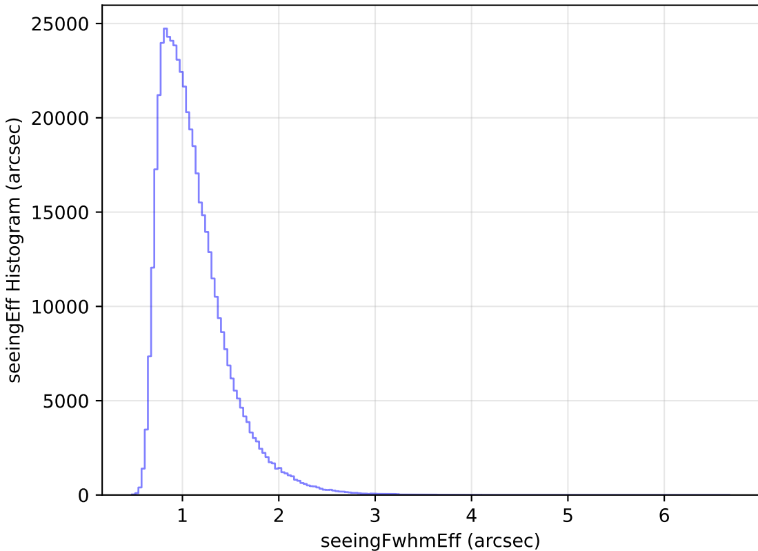
weather_cloudso2v3.4_10yrs All sky r band: seeingEff Histogram
