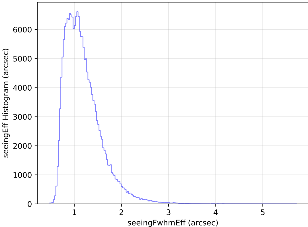
weather_cloudso2v3.4_10yrs All sky g band: seeingEff Histogram
