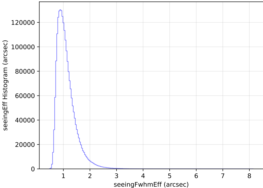
weather_cloudso2v3.4_10yrs All sky all bands: seeingEff Histogram
