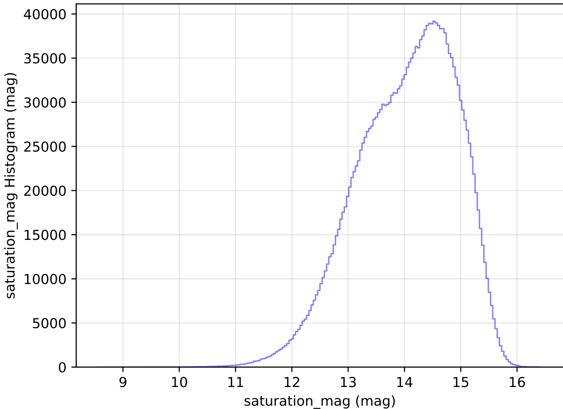
weather_cloudso2v3.4_10yrs WFD all bands: saturation_mag Histogram
