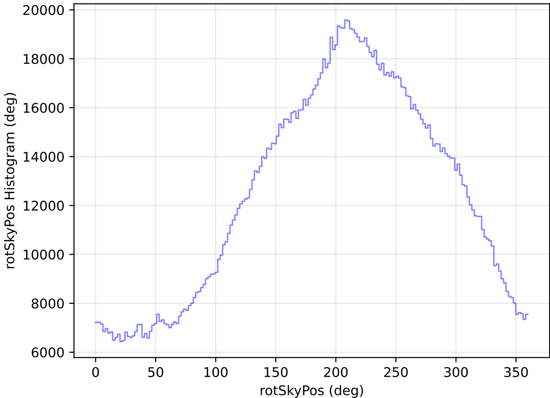
weather_cloudso2v3.4_10yrs All sky all bands: rotSkyPos Histogram
