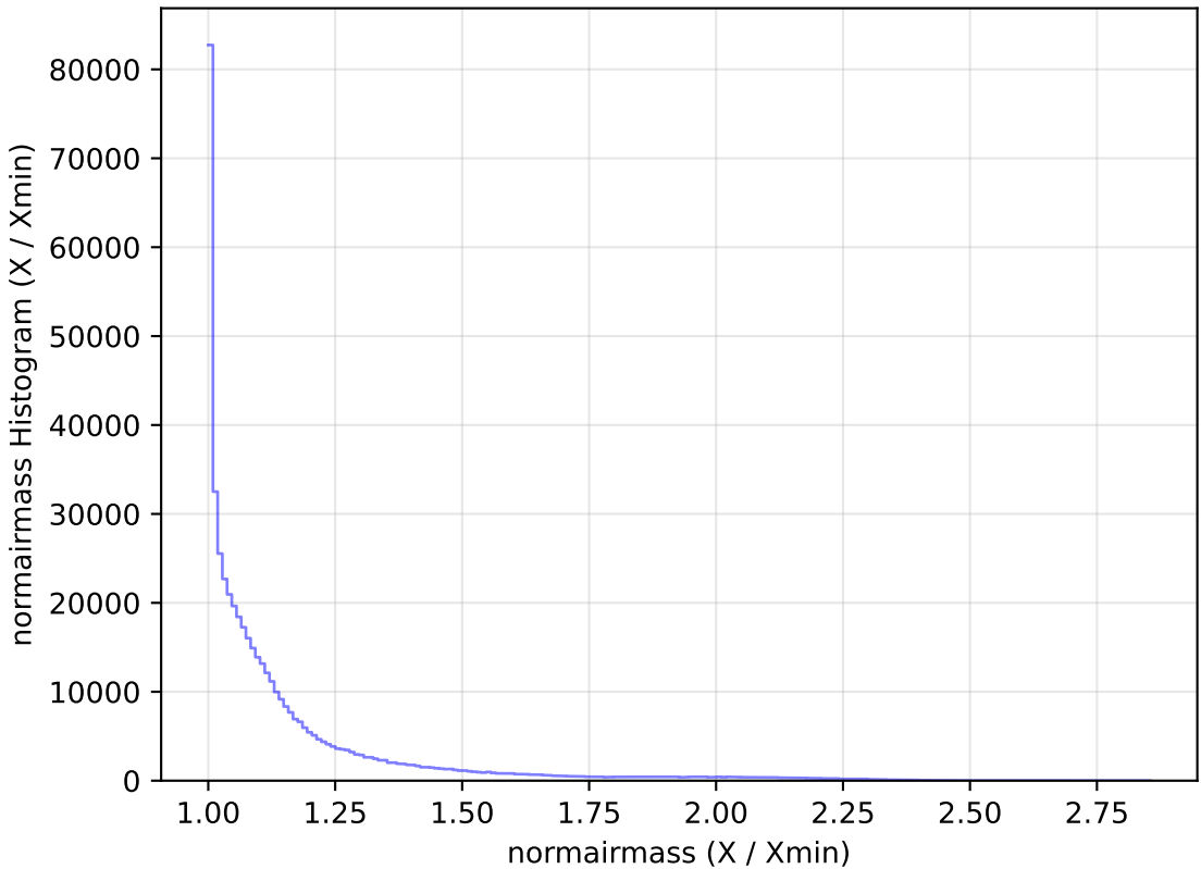
weather_cloudso2v3.4_10yrs WFD r band: normairmass Histogram
