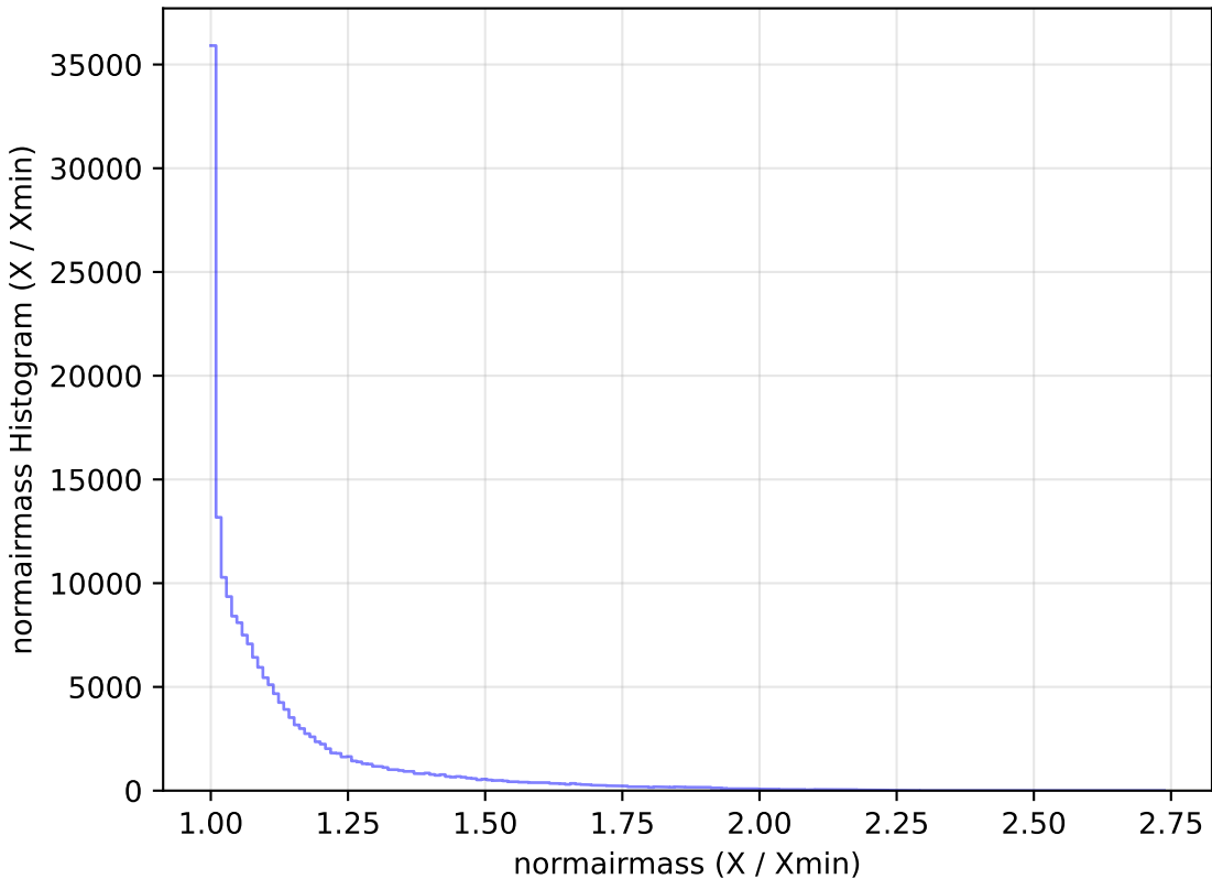
weather_cloudso2v3.4_10yrs WFD g band: normairmass Histogram
