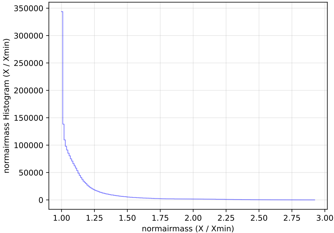
weather_cloudso2v3.4_10yrs WFD all bands: normairmass Histogram
