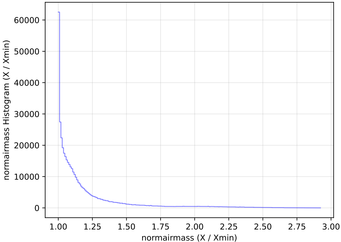
weather_cloudso2v3.4_10yrs All sky z band: normairmass Histogram
