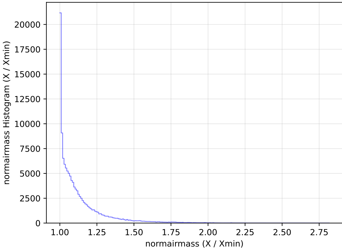
weather_cloudso2v3.4_10yrs All sky u band: normairmass Histogram
