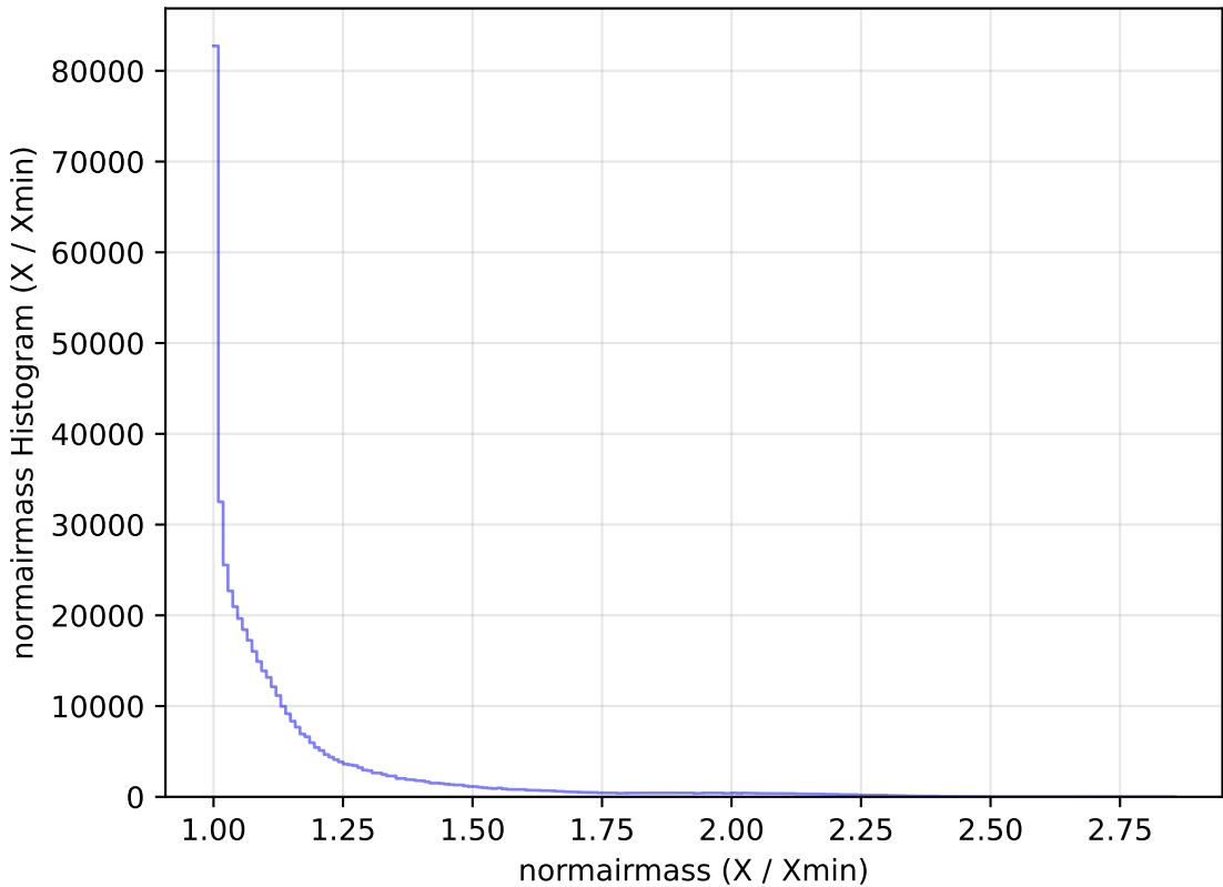
weather_cloudso2v3.4_10yrs All sky r band: normairmass Histogram
