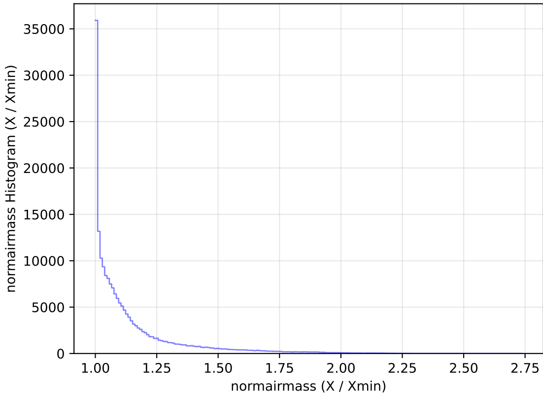
weather_cloudso2v3.4_10yrs All sky g band: normairmass Histogram
