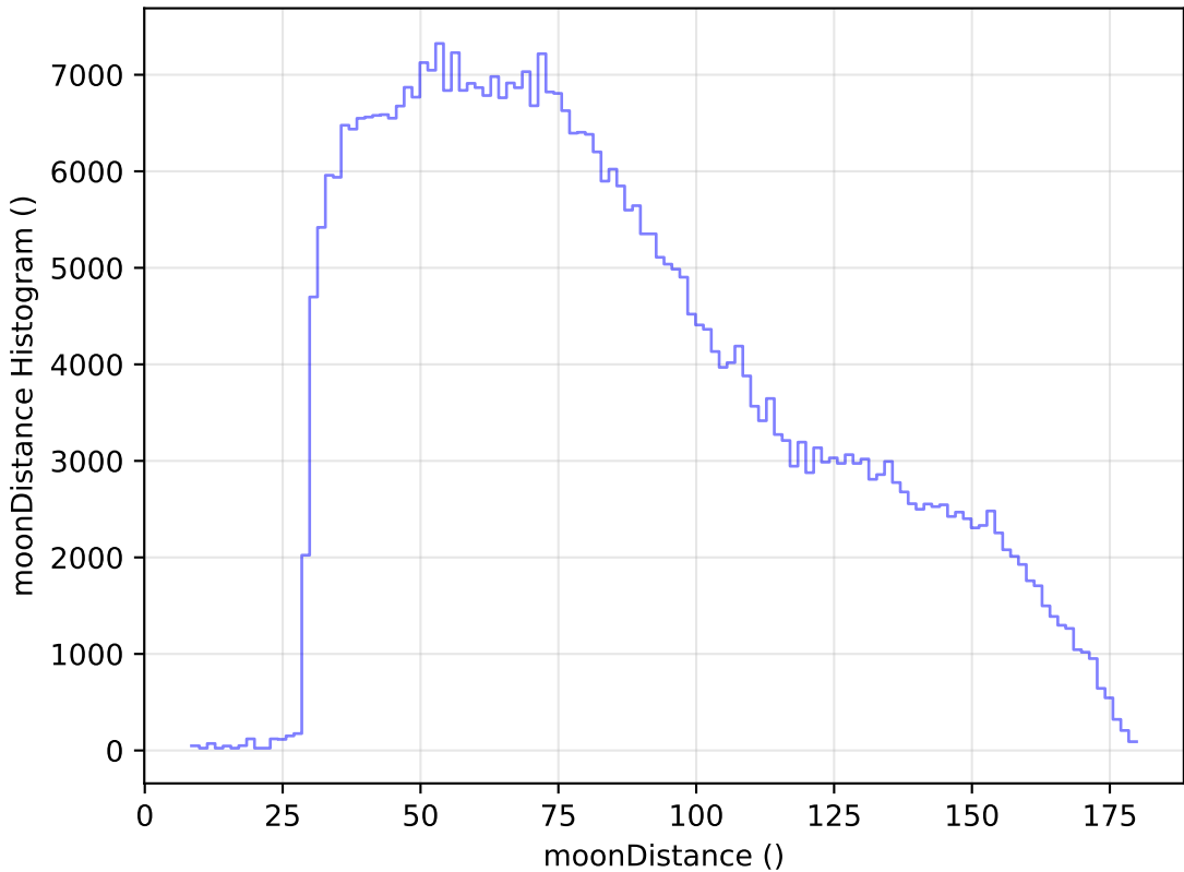
weather_cloudso2v3.4_10yrs WFD z band: moonDistance Histogram
