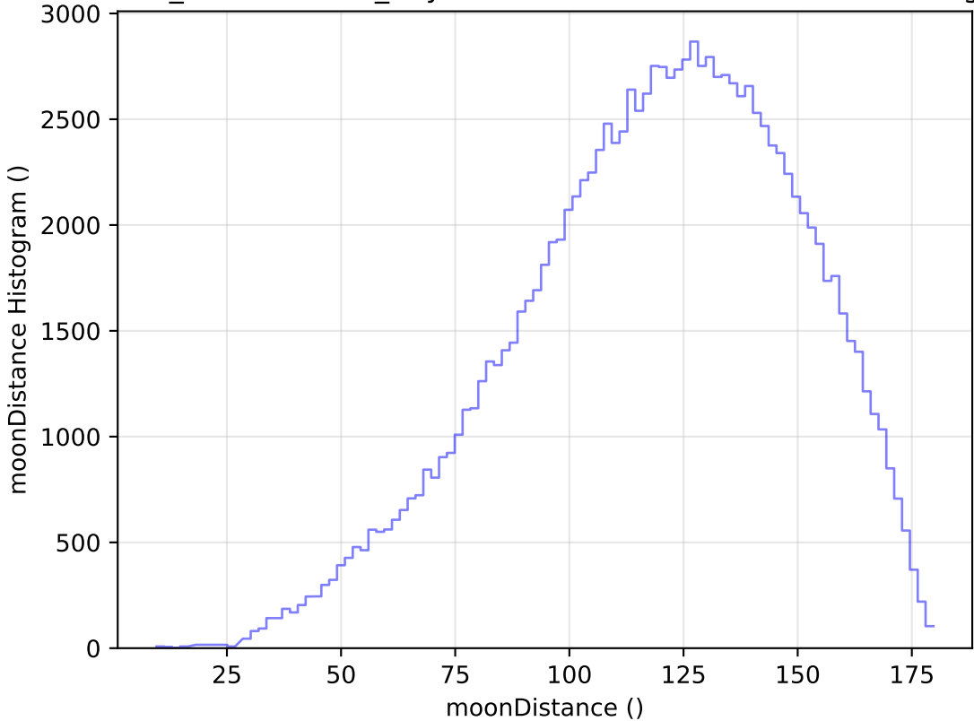
weather_cloudso2v3.4_10yrs WFD u band: moonDistance Histogram
