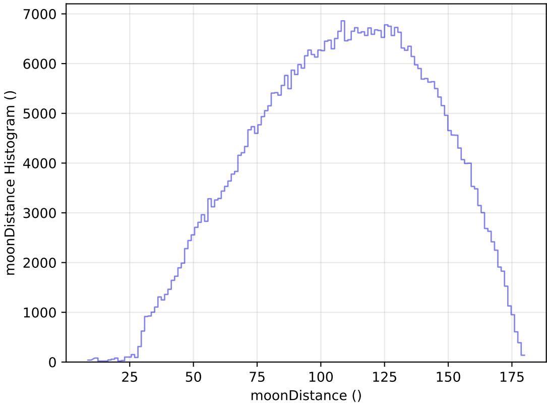
weather_cloudso2v3.4_10yrs WFD r band: moonDistance Histogram
