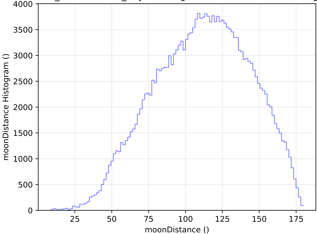
weather_cloudso2v3.4_10yrs WFD g band: moonDistance Histogram
