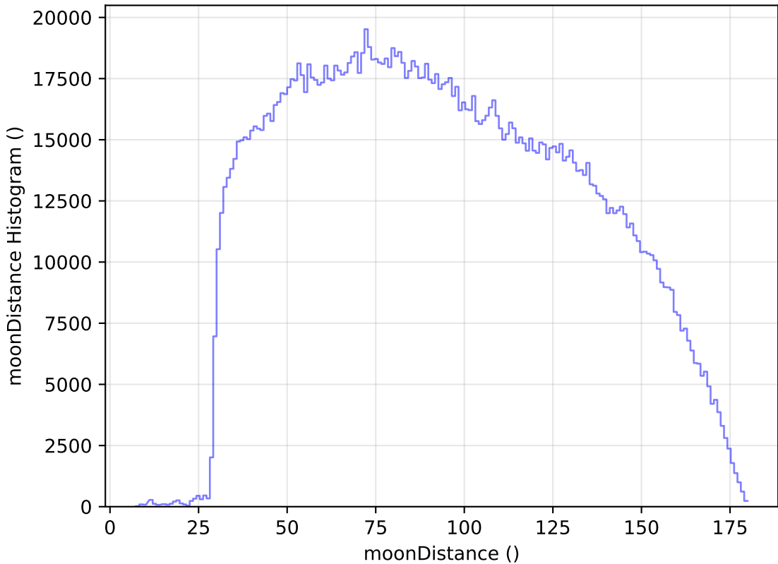
weather_cloudso2v3.4_10yrs WFD all bands: moonDistance Histogram
