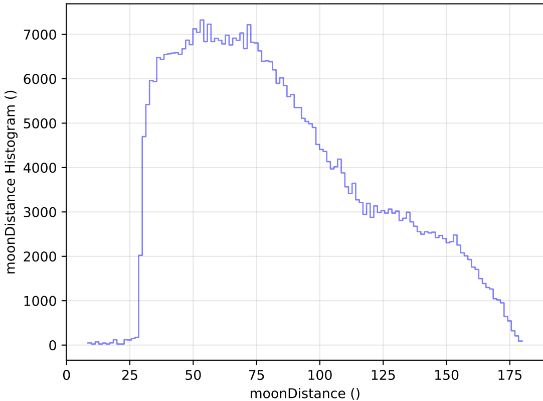
weather_cloudso2v3.4_10yrs All sky z band: moonDistance Histogram
