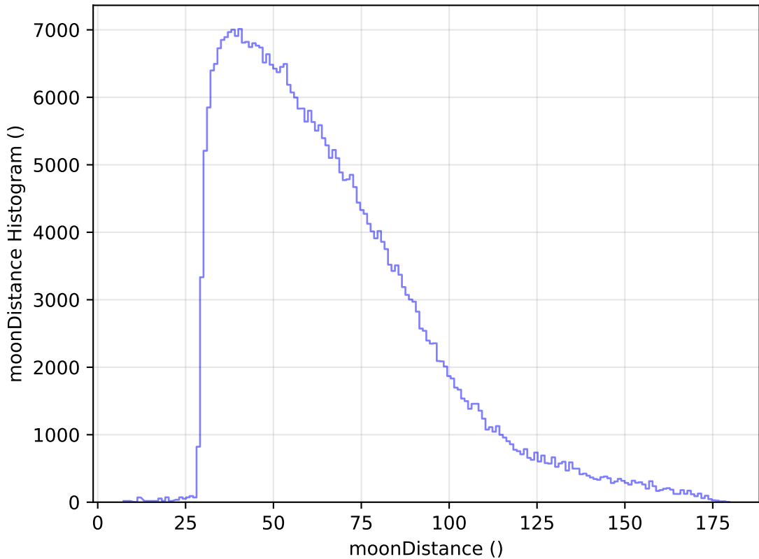
weather_cloudso2v3.4_10yrs All sky y band: moonDistance Histogram
