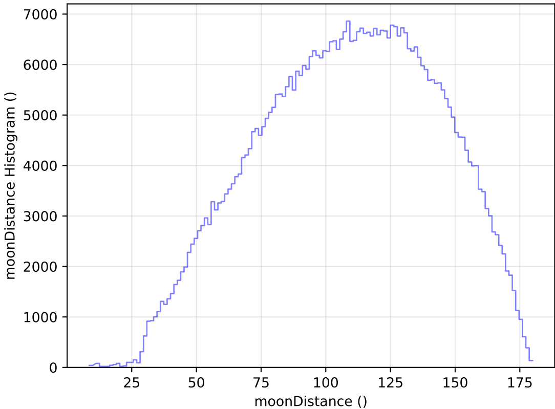
weather_cloudso2v3.4_10yrs All sky r band: moonDistance Histogram
