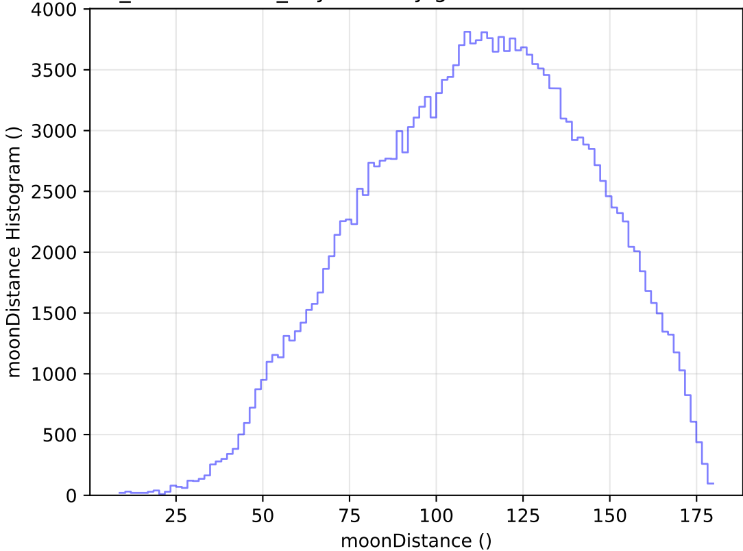
weather_cloudso2v3.4_10yrs All sky g band: moonDistance Histogram
