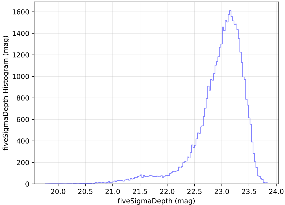
weather_cloudso2v3.4_10yrs Yr 1 z band: fiveSigmaDepth Histogram
