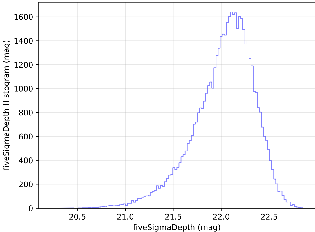
weather_cloudso2v3.4_10yrs Yr 1 y band: fiveSigmaDepth Histogram
