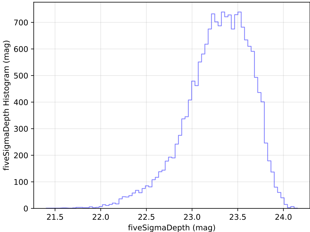
weather_cloudso2v3.4_10yrs Yr 1 u band: fiveSigmaDepth Histogram
