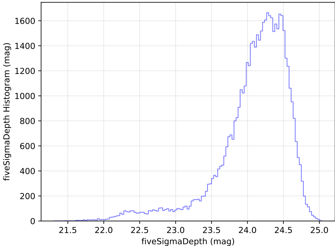
weather_cloudso2v3.4_10yrs Yr 1 r band: fiveSigmaDepth Histogram
