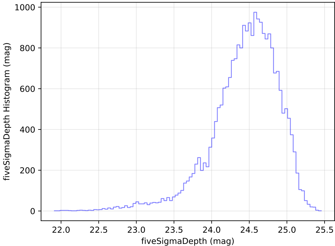
weather_cloudso2v3.4_10yrs Yr 1 g band: fiveSigmaDepth Histogram
