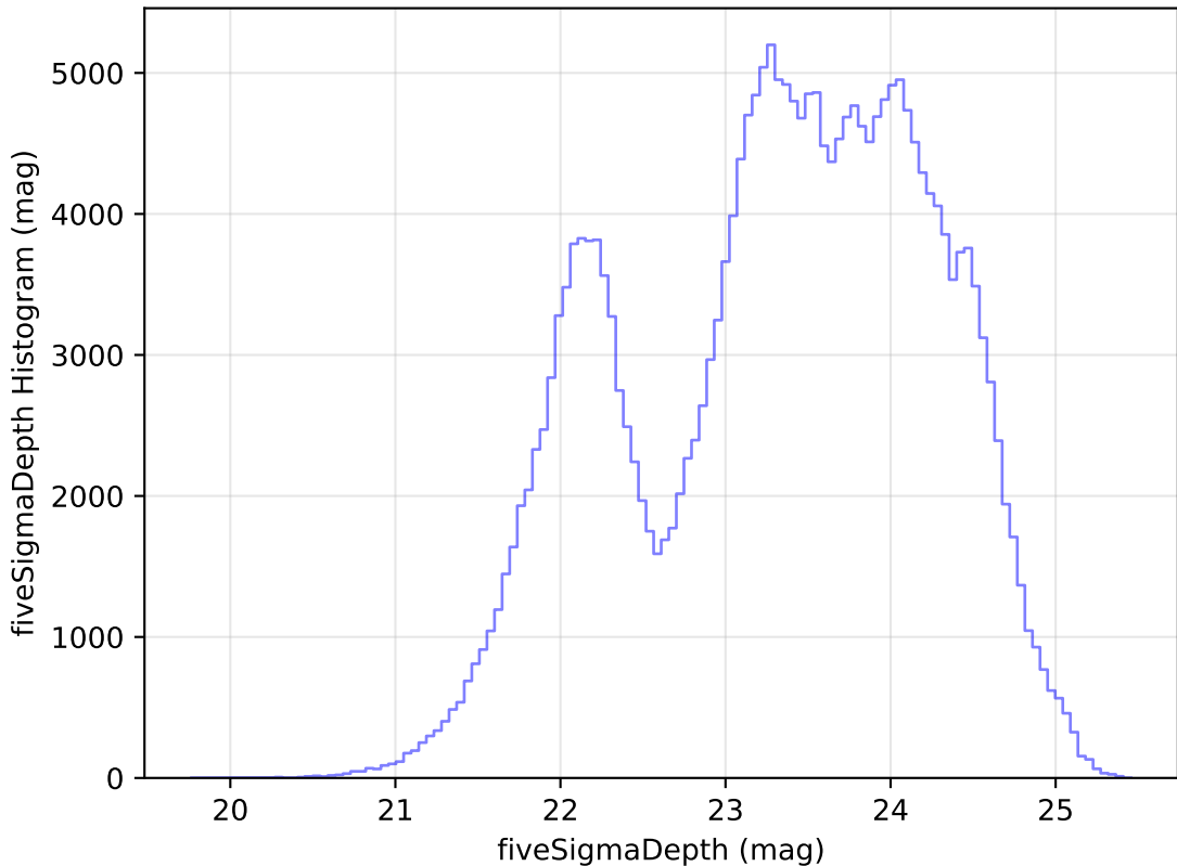
weather_cloudso2v3.4_10yrs Yr 1 all bands: fiveSigmaDepth Histogram
