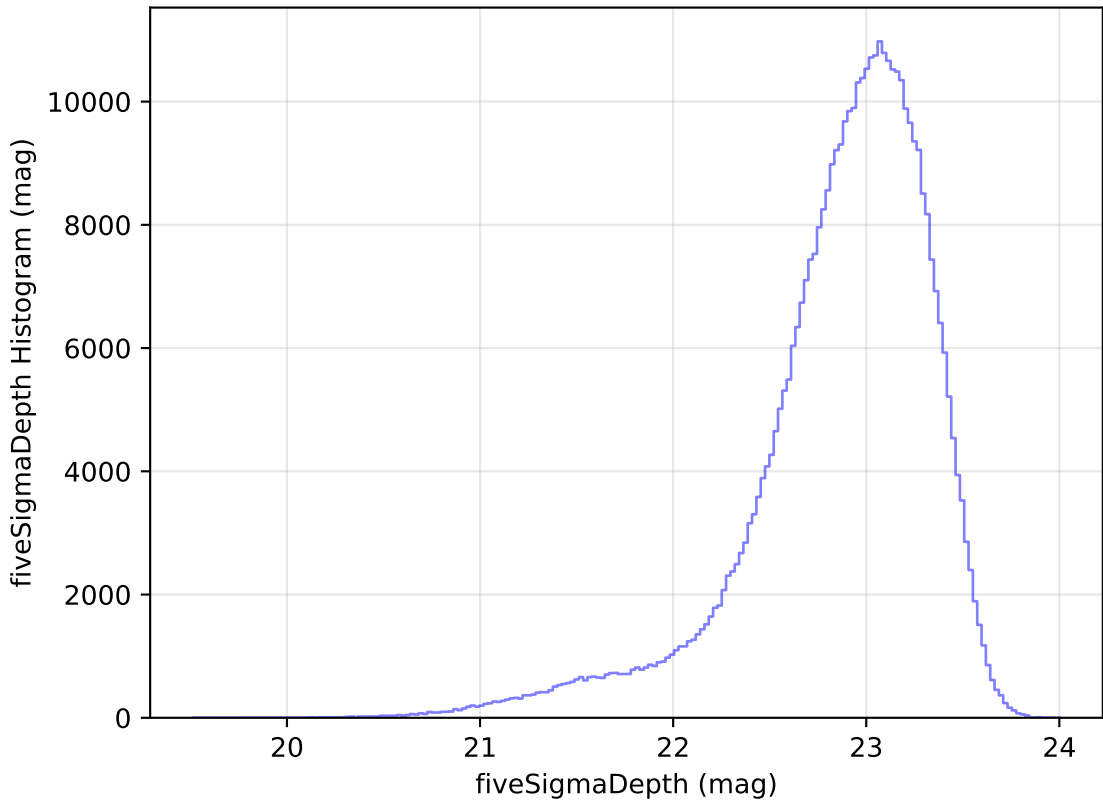
weather_cloudso2v3.4_10yrs WFD z band: fiveSigmaDepth Histogram
