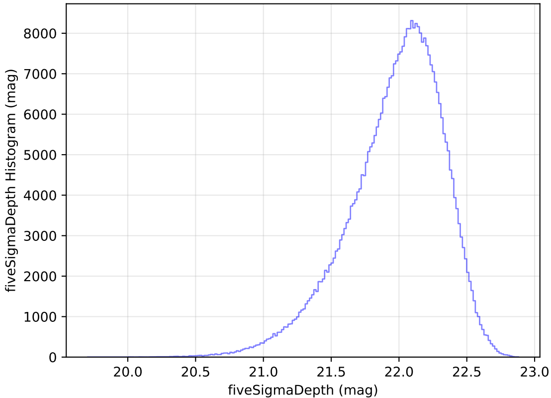
weather_cloudso2v3.4_10yrs WFD y band: fiveSigmaDepth Histogram
