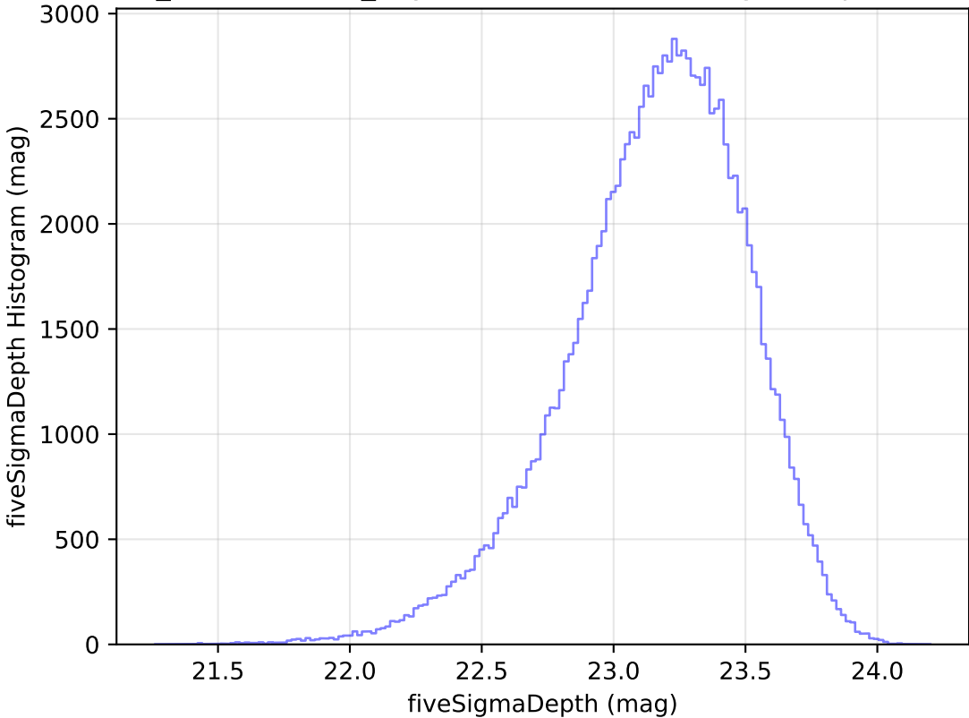
weather_cloudso2v3.4_10yrs WFD u band: fiveSigmaDepth Histogram
